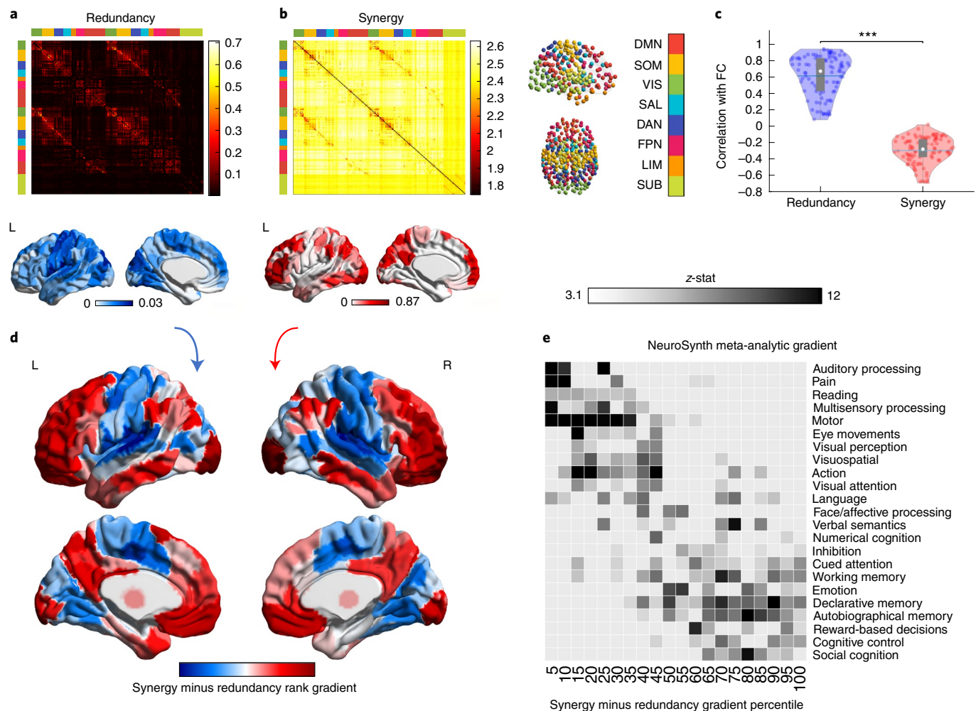
Fig. 1 | Synergistic and redundant networks exhibit distinct anatomical and cognitive profiles. a, b , Group-average matrices display the redundant ( a ) and synergistic ( b ) interactions between each pair of brain regions (note that color bars do not include entries on the diagonal). Brain plots show the cortical distribution of the strongest redundant (blue) and synergistic (red) connections (thresholded to retain the top 5% of connections, for display purposes only). SOM, somatomotor network; VIS, visual network; SAL, salience/ventral attention network; DAN, dorsal attention network; LIM, limbic network; SUB, subcortical network. c , participant-specific Pearson correlation values of synergy and redundancy matrices with the matrix of traditional FC (redundancy: M = 0.62 , s.d. = 0.24 ; synergy: M = -0.29 , s.d. = 0.16 ; t(99) = 24.06 , P < 0.001 , Hedges's g = 4.39 , effect size confidence interval (CI): (3.88, 5.11), from paired-sample non-parametric permutation t -test (two-sided); n = 100 unrelated HCP participants). Note that the relationships of redundancy and synergy with traditional FC are not equal: the absolute value of the correlation was significantly stronger for redundancy than for synergy (redundancy: M = 0.62 , s.d. = 0.24 ; synergy: M = 0.29 , s.d. = 0.16 ; t(99) = 20.35 , P < 0.001 , Hedges's g = 1.65 , effect size CI: (1.36, 1.92), from paired-sample non-parametric permutation t -test (two-sided); n = 100 unrelated HCP participants). In the violin plots, each colored circle represents one participant; white circle, median; blue line, mean; box limits, upper and lower quartiles; whiskers, 1.5 \times interquartile range; *** P < 0.001 . d , Brain surface projections of regional redundancy-to-synergy gradient scores, based on the respective ranks. These ranks exhibited an inverse correlation (Spearman's \rho = -0.40 , P < 0.001 ; Extended Data Fig. 1). e , NeuroSynth term-based meta-analysis, relating the distribution of redundancy-to-synergy gradient across the brain to a cognitive gradient of cognitive domains, from lower-level sensorimotor processing to higher-level cognitive tasks. These results are robust to the use of different parcellations (cortical only; having lower or higher number of nodes; and obtained from anatomical rather than functional considerations; Extended Data Fig. 2a,b). Likewise, although these results were obtained after deconvolving the hemodynamic response function from the BOLD signals to account for regional variations (Methods), analogous results are also obtained when this step is omitted, or if synergy and redundancy are computed from discretized rather than continuous data (Extended Data Fig. 2c,d).
