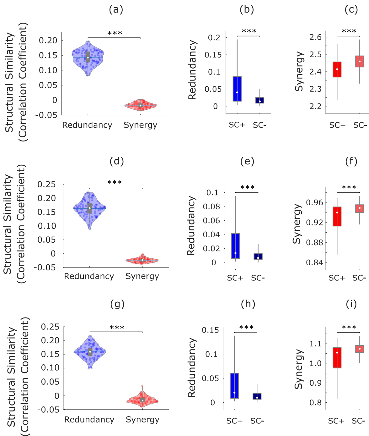
Extended Data Fig. 4 | Robustness of synergy and redundancy structure-function results to alternative node and edge definitions. (a-c) Robustness of structure-function results to the use of the 308-ROI cortical parcellation. (d-f) Robustness of structure-function results to using synergy and redundancy normalised by TDMI. (g-i) Robustness of structure-function results to using synergy and redundancy obtained from discretised signals. For all violin plots: each colored circle represents one subject; white circle: median; central line: mean; box limits, upper and lower quartiles; whiskers, 1.5x inter-quartile range; *** p < 0.001 from paired-sample non-parametric permutation t-test (two-sided); n = 100 unrelated HCP subjects. For all box-plots: white circle: median; box limits, upper and lower quartiles; whiskers, 1.5x inter-quartile range; *** p < 0.001 from two-sample non-parametric permutation t-test (two-sided). For (b-c), SC+, n=6864 direct connections; SC-, n=88000 connections. For (e-f) and (h-i), SC+, n=5276 direct connections; SC-, n=48548 indirect connections.
