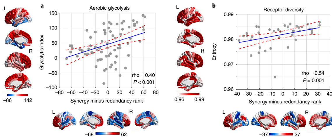
Fig. 7 | Metabolic and molecular underpinnings of synergy in the human brain. a , Significant Spearman correlation (two-sided CI: 0.195, 0.572) between regional redundancy-to-synergy gradient scores, and the mean regional estimate of AG based on PET measurements of cerebral metabolic rates for oxygen and glucose (GI); n = 78 cortical regions. b , Significant Spearman correlation (two-sided CI: 0.270, 0.731) between cortical redundancy-to-synergy gradient scores, and the diversity (entropy) of neurotransmitter receptor expression from in vitro quantitative autoradiography across n = 39 regions of human visual, somatosensory, auditory and multimodal association cortices. Colored bars correspond to scatterplot axes.
