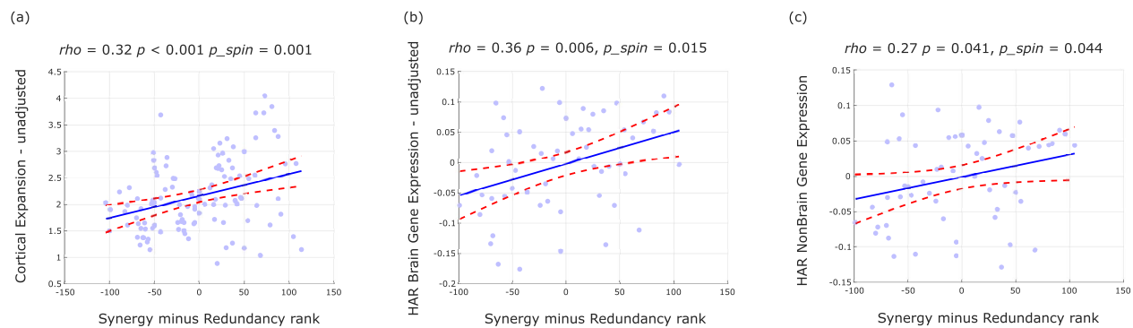
Extended Data Fig. 8 | Synergy-redundancy gradient correlates with unadjusted cortical expansion and gene expression. (a) Significant Spearman correlation (two-sided CI: [0.145, 0.476]) between regional redundancy-to-synergy gradient scores and unadjusted regional cortical expansion from chimpanzee ( Pan troglodytes ) to human (both on DK-114 cortical atlas, both hemispheres; n=114 cortical regions). (b) Significant Spearman correlation (two-sided CI: [0.109, 0.567]) between regional redundancy-to-synergy gradient scores and unadjusted regional expression of brain-related human-accelerated (HAR) genes (both on left hemisphere of DK-114 atlas; n=57 left-hemisphere regions). (c) Significant Spearman correlation (two-sided CI: [0.010, 0.496]) between regional redundancy-to-synergy gradient scores and unadjusted regional expression of non-brain-related human-accelerated (HAR) genes (both on left hemisphere of DK-114 atlas; n=57 left-hemisphere regions). p_{spin} indicates the p-value estimated from a spatial permutation test comparing the empirical correlation against 10,000 randomly rotated brain maps with preserved spatial covariance.
