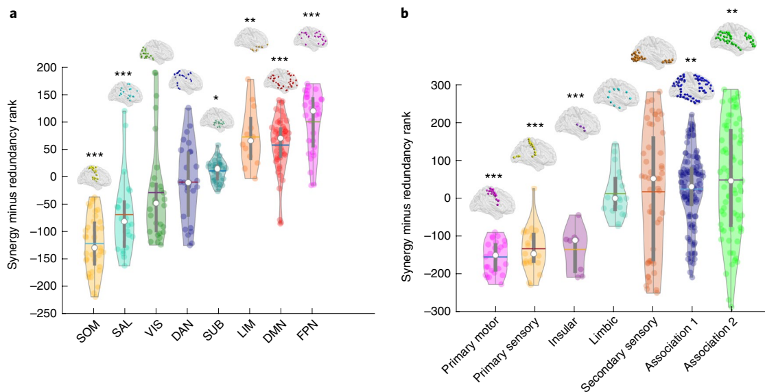
Fig. 2 | Distinct cytoarchitectonic and resting-state network profiles for synergy-dominated and redundancy-dominated regions. a, Regional redundancy-to-synergy gradient values for each canonical resting-state network, based on the definition of Yeo et al. 24 . b, Regional redundancy-to-synergy gradient values for each of seven cytoarchitectonic classes (the five canonical classes identified by Von Economo, plus limbic and insular cortices), for 308 cortical regions of interest (ROIs) of equal size (500 mm 2 ), obtained from subdivisions of the Desikan–Killiany cortical parcellation 23 . Each colored circle represents one brain region; n = 232 regions divided into eight resting-state networks ( a ); n = 308 regions divided into seven cytoarchitectonic classes ( b ). Each violin plot shows the distribution of brain regions assigned to the subnetwork or cytoarchitectonic class indicated on the x axis (each region is assigned exactly once). White circles represent median values, central lines represent the mean values, box limits represent upper and lower quartiles and whiskers represent 1.5x the interquartile range; * P < 0.05 , ** P < 0.01 and *** P < 0.001 , from one-sample non-parametric permutation t -test (two-sided), corrected for multiple comparisons using the false discovery rate (FDR). Full statistical results are shown in Supplementary Tables 1 (Yeo RSN) and 2 (Von Economo).
