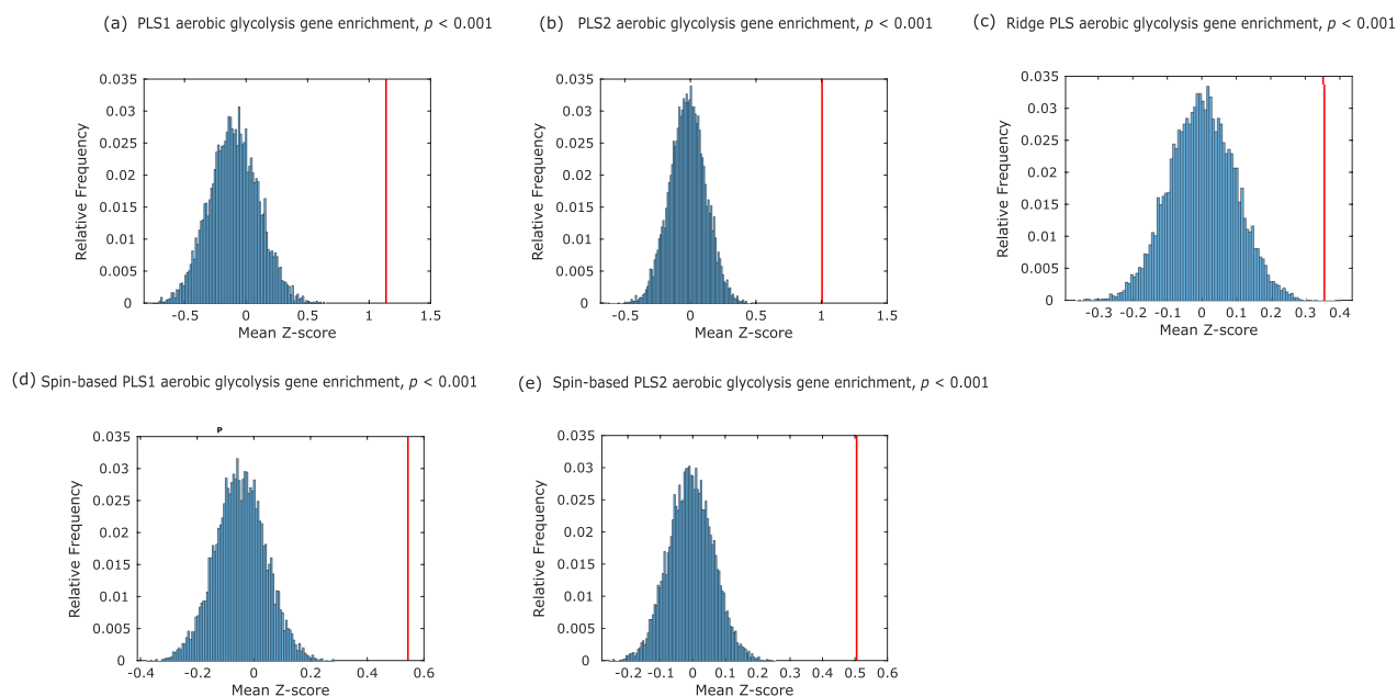
Extended Data Fig. 10 | Enrichment analysis for genes pertaining to synaptic formation, whose regional distribution corresponds to the distribution of aerobic glycolysis in the human brain, as reported by Goyal et al. (2014) ('aerobic glycolysis genes'). (a,b) PLS1 and PLS2 are significantly enriched for aerobic glycolysis genes. (c) Enrichment for genes related to aerobic glycolysis is also observed using an alternative approach: ridge-regularised PLS regression on the binarised cortical pattern of synergy vs redundancy prevalence. (d,e) Significant enrichment for genes related to aerobic glycolysis in PLS1 and PLS2 is also observed when controlling for spatial autocorrelation using spin-based permutations. (a-e) Statistical significance is assessed via bootstrap resampling of Z-scores; histograms indicate the relative frequency (over 1,000 bootstraps) of the mean Z-score of a random sample of genes of equal size as the aerobic glycolysis genes. Red vertical line: empirical mean Z-score of aerobic glycolysis genes.
