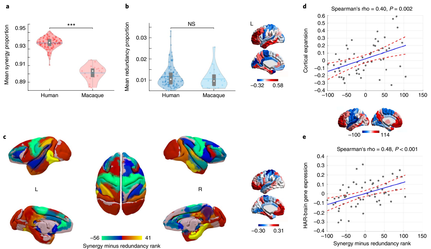
Fig. 5 | Human brain evolution favored high synergy. a , The proportion of synergistic interactions across the brain was significantly higher in humans ( H. sapiens ) than in macaques ( M. mulatta ; human M = 0.937 , s.d. = 0.007 ; macaque M = 0.901 , s.d. = 0.009 ; t(117) = 19.86 , P < 0.001 , Hedges's g = 4.94 , effect size CI: (4.12, 6.10), from two-sample non-parametric permutation t -test (two-sided). Human data: n = 100 unrelated HCP participants. Macaque data: n = 19 distinct sessions from ten individual macaques). b , The proportion of redundant interactions across the brain was equivalent in humans and macaques (redundancy: human M = 0.012 , s.d. = 0.005 ; macaque M = 0.011 , s.d. = 0.005 ; t(117) = 0.90 , P = 0.372 , Hedges's g = 0.22 , effect size CI: (-0.28, 0.66), from two-sample non-parametric permutation t -test (two-sided). Human data: n = 100 unrelated HCP participants. Macaque data: n = 19 distinct sessions from ten individual macaques). White circles represent median values, central lines represent the mean values, box limits represent upper and lower quartiles and whiskers represent 1.5 \times the interquartile range; *** P < 0.001 ; NS, not significant P > 0.05 . Note that the proportion of synergy can differ even if the proportion of redundancy remains the same; as mentioned in the introduction, synergy and redundancy are not the only constituent elements of total information flow in the system: each source (here, brain region) also brings a unique contribution 26 . The results presented here cannot be solely attributed to either the choice of bandpass filter or the difference in TR between datasets (Extended Data Fig. 6). The proportion of synergistic information was significantly higher in humans than macaques even when the comparison was restricted only to those humans whose total FC strength was in the range of the macaque values (Extended Data Fig. 6). c , Surface projection of regional redundancy-to-synergy gradient scores for the macaque brain. Corresponding matrices of synergy and redundancy are shown in Extended Data Fig. 7. d , Significant Spearman correlation (two-sided CI: (0.16, 0.59)) between human regional redundancy-to-synergy gradient scores and regional cortical expansion from chimpanzee ( P. troglodytes ) to human ( n = 57 regions of the left hemisphere of the DK-114 atlas). This result is not due to spatial autocorrelation, as assessed using spin-based permutation testing; P_{\text{spin}} = 0.010 . e , Significant Spearman correlation (two-sided CI: (0.25, 0.66)) between human regional redundancy-to-synergy gradient scores and regional expression of brain-related human-accelerated (HAR-Brain) genes ( n = 57 regions of the left hemisphere of the DK-114 atlas). This result is not due to spatial autocorrelation, as assessed using spin-based permutation testing; P_{\text{spin}} = 0.002 . These results are also robust to the use of unadjusted scores (Extended Data Fig. 8).
