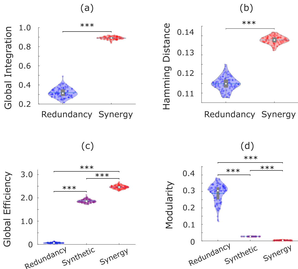
Extended Data Fig. 5 | Additional validation of synergy and redundancy network results. (a) Alternative measure of global integration (area under the curve of the size of the largest connected component across thresholds). (b) Alternative structural-functional dissimilarity (mean Hamming distance). For both (a) and (b): *** p < 0.001 from paired-sample non-parametric permutation t-test (two-sided), n=100 unrelated HCP subjects. (c) Comparison of global efficiency of synergy and redundancy networks of each subject with the average global efficiency of 100 synthetic null networks with edges randomly drawn from the distribution between 0 and the empirical TDMI. (d) Comparison of modularity of synergy and redundancy networks of each subject with the average modularity of 100 synthetic null networks with edges randomly drawn from the distribution between 0 and the empirical TDMI. For (c) and (d), *** p < 0.001 (FDR-corrected) from two-sample non-parametric permutation t-test (two-sided); n = 100 unrelated HCP subjects and n=100 synthetic null networks. For all violin plots: each colored circle represents one subject; white circle: median; central line: mean; box limits, upper and lower quartiles; whiskers, 1.5x inter-quartile range.
