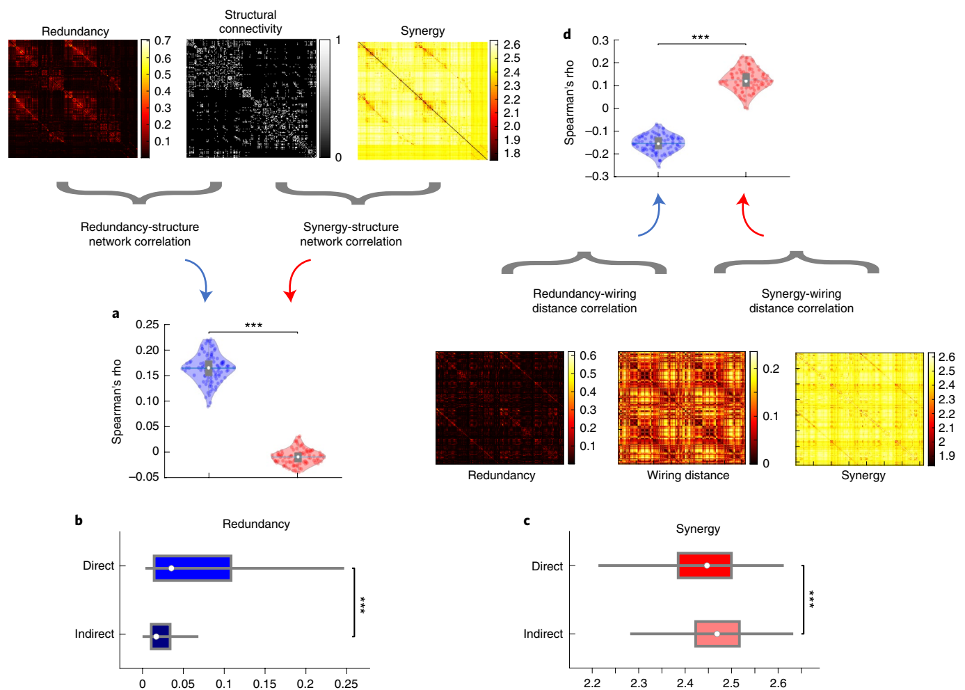
Fig. 4 | Redundant interactions are supported by anatomical connections; synergistic interactions connect regions with distinct structural wiring profiles.
