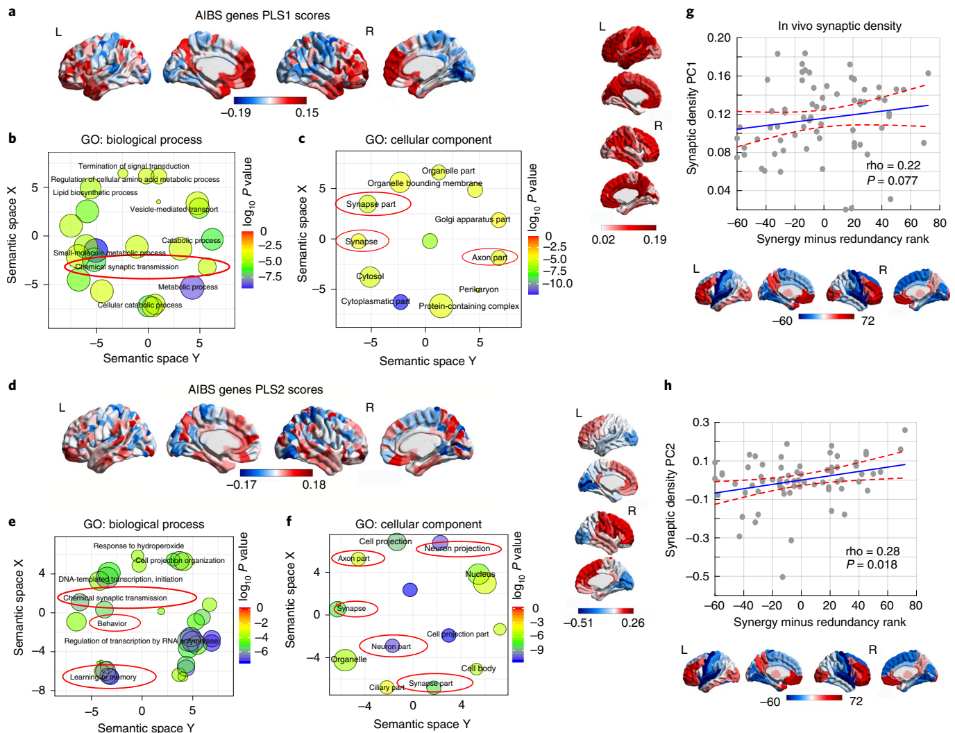
Fig. 6 | Synaptic underpinnings of synergy in the human brain. a , First principal component of PLS (PLS1) relating the redundancy-to-synergy regional gradient to n=20,647 genes from the AIBS. b,c , Dimensionality-reduced GO terms pertaining to biological processes ( b ) or cellular components ( c ) that are significantly enriched in PLS1, obtained from GOrilla using the 'P-value threshold 10^{-4} ' setting to best approximate FDR correction with \alpha=0.05 (ref. 35 ) and summarized with REVIGO (added red ovals highlight psychologically or neurobiologically relevant terms). Semantic space axes indicate the relative distance between terms in multidimensional space, but have no intrinsic meaning. d , Second principal component of PLS (PLS2) relating the redundancy-to-synergy regional gradient to n=20,647 genes from the AIBS. e,f , Dimensionality-reduced GO terms pertaining to biological processes ( e ) or cellular components ( f ) that are significantly enriched in PLS2, obtained from GOrilla using the 'P-value threshold 10^{-4} ' setting to best approximate FDR correction with \alpha=0.05 (ref. 35 ) and summarized with REVIGO (added red ovals highlight psychologically or neurobiologically relevant terms). These results are robust to the use of alternative approaches (ridge-regularized PLS regression on the synergy–redundancy cortical pattern; and controlling for spatial autocorrelation using spin-based permutations 53 ; Extended Data Fig. 9). The significant enrichment for synaptic transmission and organization was also preserved when using recently developed advanced null models based on random phenotype ensembles (Supplementary Table 10). g , Spearman correlation between regional redundancy-to-synergy gradient scores and the first principal component of in vivo synaptic density from [ ^{11} C]UCB-J PET (Spearman \rho=0.22 , p=0.077 ; two-sided CI: -0.019, 0.436; P_{\text{spin}}=0.053 ; n=68 cortical regions). Colored bars correspond to scatterplot axes. h , Spearman correlation between regional redundancy-to-synergy gradient scores and the second (anteroposterior) principal component of in vivo synaptic density from [ ^{11} C]UCB-J PET (Spearman \rho=0.28 , p=0.018 ; two-sided CI: 0.044, 0.486; P_{\text{spin}}=0.059 ; n=68 cortical regions). Colored bars correspond to scatterplot axes.
