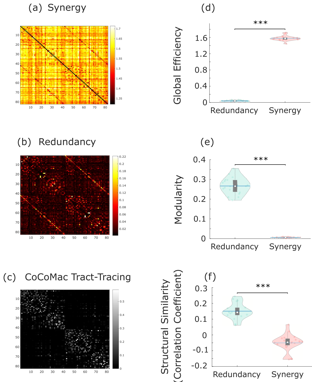
Extended Data Fig. 7 | Characterisation of synergistic and redundant network profiles in macaque brains are similar to humans. (a) Synergistic interactions between regions of the macaque brain. (b) Redundant interactions between regions of the macaque brain. (c) Anatomical connectivity was estimated from axonal tracing and diffusion MRI (Shen et al. , 2019), and Spearman correlation coefficient was used to assess the similarity of redundancy and synergy matrices with structural connectivity, after thresholding to ensure equal numbers of connections. (d) The network organisation of synergistic interactions exhibits significantly higher global efficiency than redundant interactions ( p < 0.001 ). (e) The network organisation of redundant interactions exhibits significantly higher segregation (modularity) than synergistic interactions ( p < 0.001 ). (f) Networks of redundant interactions are significantly more correlated with underlying anatomical connectivity than synergistic interactions ( p < 0.001 ). For all tests: *** p < 0.001 from paired-sample non-parametric permutation t-test (two-sided); n=19 distinct sessions from 10 individual macaques (Supplementary Table 7). For all violin plots: each colored circle indicates one data-point; white circle: median; central line: mean; box limits, upper and lower quartiles; whiskers, 1.5x inter-quartile range.
