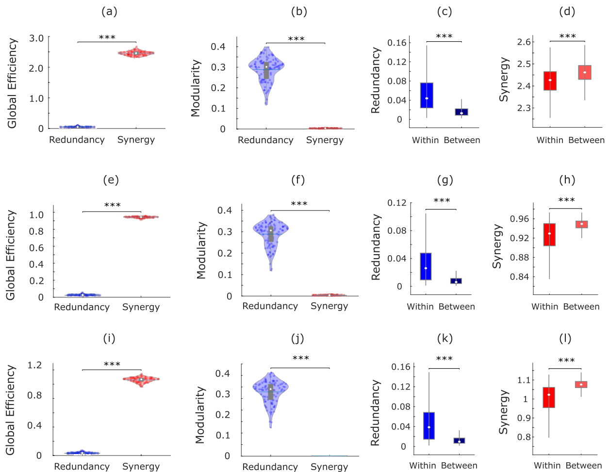
Extended Data Fig. 3 | Robustness of synergy and redundancy network results (efficiency, modularity, and within- vs between-resting state subnetwork comparison) to alternative node and edge definitions. (a-d) Robustness of network results to the use of the 308-ROI cortical parcellation. (e-h) Robustness of network results to using synergy and redundancy normalised by TDMI. (i-l) Robustness of network results to using synergy and redundancy obtained from discretised signals. For all violin plots: each colored circle represents one subject; white circle: median; central line: mean; box limits, upper and lower quartiles; whiskers, 1.5x inter-quartile range; *** p < 0.001 from paired-sample non-parametric permutation t-test (two-sided); n = 100 unrelated HCP subjects. For all box-plots: white circle, median; box limits, upper and lower quartiles; whiskers, 1.5x inter-quartile range; *** p < 0.001 from two-sample non-parametric permutation t-test (two-sided). For (c-d) and (k-l), Within-RSN n=7178 connections; Between-RSN n=46414 connections. For (g) and (h), Within-RSN n=14784 connections; Between-RSN n=79772 connections.
