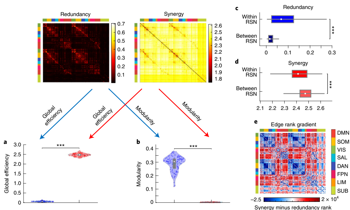
Fig. 3 | Network analysis indicates global and segregated processing for synergy and redundancy, respectively. a , The whole-brain network organization of synergistic interactions exhibited significantly higher global efficiency than the whole-brain network of redundant interactions (synergy: M = 2.47 , s.d. = 0.08 ; redundancy: M = 0.07 , s.d. = 0.02 ; t(99) = -285.75 , P < 0.001 , Hedges's g = -43.58 , effect size CI: (-50.46, -38.75) , from paired-sample non-parametric permutation t -test (two-sided); n = 100 unrelated HCP participants). b , The whole-brain network of redundant interactions exhibited significantly higher segregation (modularity) than the network of synergistic interactions (synergy: M = 0.003 , s.d. = 0.001 ; redundancy: M = 0.29 , s.d. = 0.05 ; t(99) = 52.12 , P < 0.001 , Hedges's g = 7.28 , effect size CI: (6.22, 8.85) , from paired-sample non-parametric permutation t -test (two-sided); n = 100 unrelated HCP participants). For the violin plots, each colored circle represents one participant; white circles represent median values, central lines represent the mean values, box limits represent upper and lower quartiles and whiskers represent 1.5 \times the interquartile range; ***P < 0.001 . c , Redundant connections were significantly stronger within functional resting-state subnetworks (RSNs) than between them (within-RSN: M = 0.087 , s.d. = 0.078 , n = 7,178 within-RSN connections; between-RSN: M = 0.026 , s.d. = 0.027 , n = 46,414 between-RSN connections; t(53,590) = 127.45 , P < 0.001 , Hedges's g = 1.61 , effect size CI: (1.58, 1.66) ; from two-sample non-parametric permutation t -test (two-sided)). d , Synergistic connections were significantly stronger between functional resting-state subnetworks than within them (within-RSN: M = 2.41 , s.d. = 0.09 , n = 7,178 within-RSN connections; between-RSN: M = 2.47 , s.d. = 0.06 , n = 46,414 between-RSN connections; t(53,590) = -75.31 , P < 0.001 , Hedges's g = -0.96 , effect size CI: (-0.99, -0.92) ; from two-sample non-parametric permutation t -test (two-sided)). For the box plots, white circles represent the median values; box limits the upper and lower quartiles and whiskers represent 1.5 \times the interquartile range. e , Matrix of redundancy-to-synergy gradient scores for each connection between brain regions, highlighting regions' affiliation with the resting-state subnetworks of Yeo et al. 24 . Red indicates synergy > redundancy. These results are robust to the use of alternative ways of defining nodes and edges, and alternative network measures (Extended Data Figs. 3–5 and Supplementary Tables 3 and 4).
