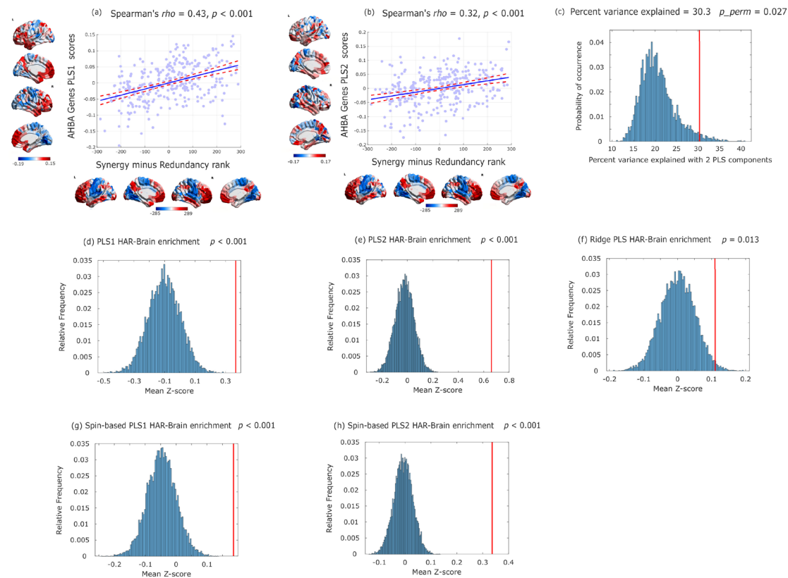
Extended Data Fig. 9 | Characterisation of PLS components of 20,647 genes from the Allen Institute for Brain Science, for the 308-ROI subdivision of the Desikan-Killiany cortical parcellation. (a) Spearman correlation (two-sided CI: [0.334, 0.517]; n=308 regions) between the redundancy-to-synergy regional pattern, and the first principal component of PLS (PLS1). (b) Spearman correlation (two-sided CI: [0.216, 0.417]; n=308 regions) between the redundancy-to-synergy regional pattern, and the second principal component of PLS (PLS2). For both (a) and (b), color-bars correspond to scatter-plot axes. (c) The variance explained by the first 2 PLS components is significantly higher than would be expected based on random patterns with preserved spatial autocorrelation, assessed using spin-based permutations (Methods). (d,e) Significant enrichment of HAR-Brain genes in PLS1 and PLS2. (f) Significant HAR-Brain gene enrichment is also observed using an alternative approach: ridge-regularized PLS regression on the binarised cortical pattern of synergy vs redundancy prevalence. (g,h) HAR-Brain gene enrichment in PLS1 and PLS2 is also observed when controlling for spatial autocorrelation using spin-based permutations. (c-h) Statistical significance is assessed via bootstrap resampling of Z-scores; histograms indicate the relative frequency (over 1,000 bootstraps) of the mean Z-score of a random sample of genes of equal size as the HAR-Brain genes. Red vertical line: empirical mean Z-score of HAR-Brain genes.
